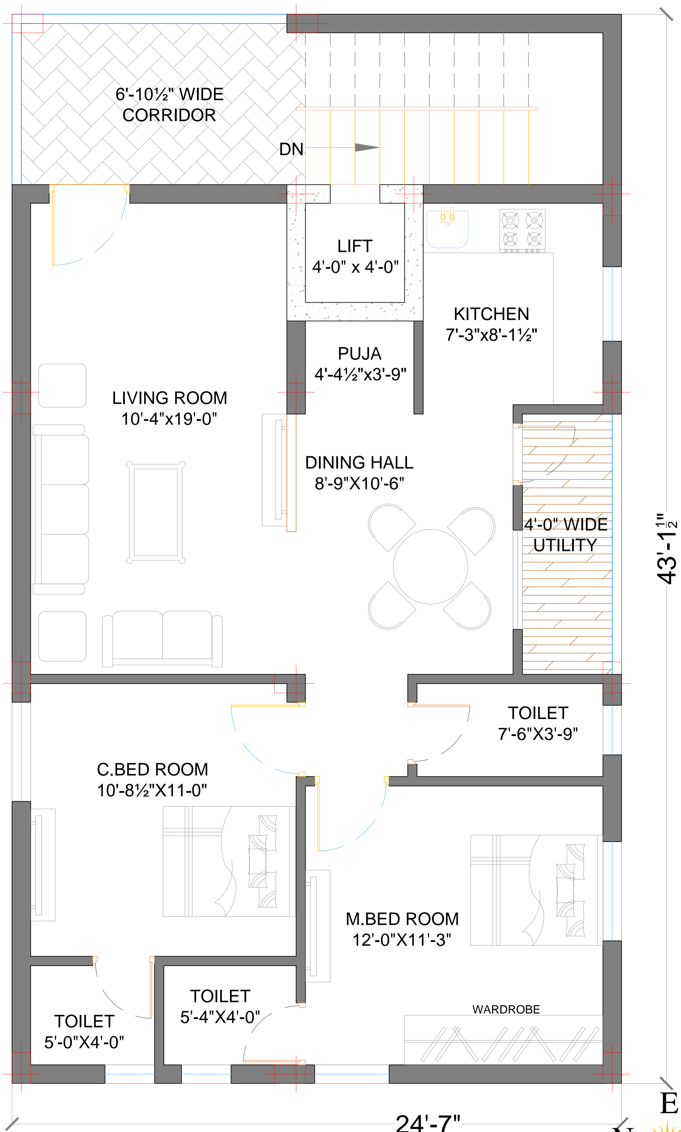
03 FIRST FLOOR PLAN SCALE-NTS
